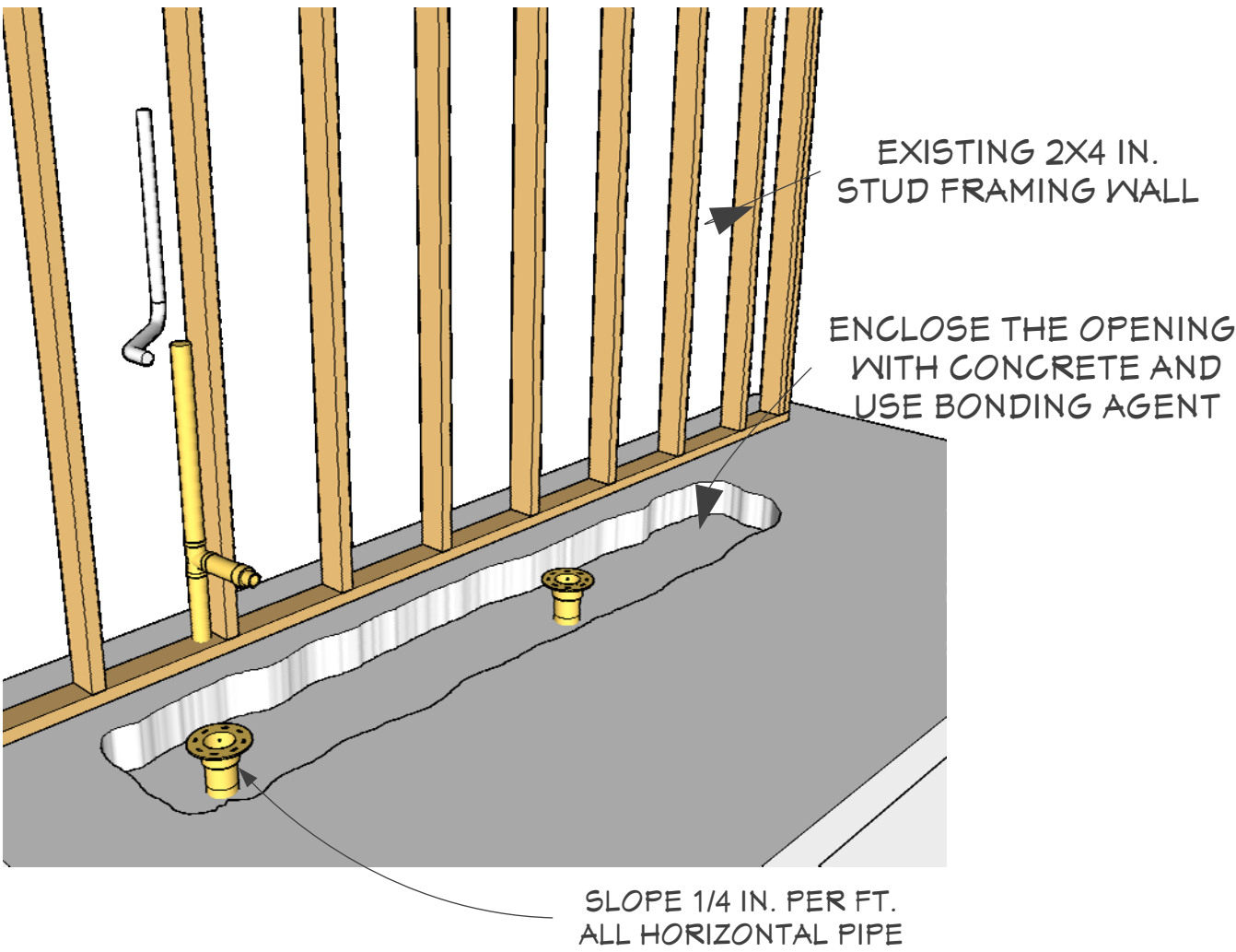
PLUMBING UNDERGROUND PIPE DETAIL (TYP.)
