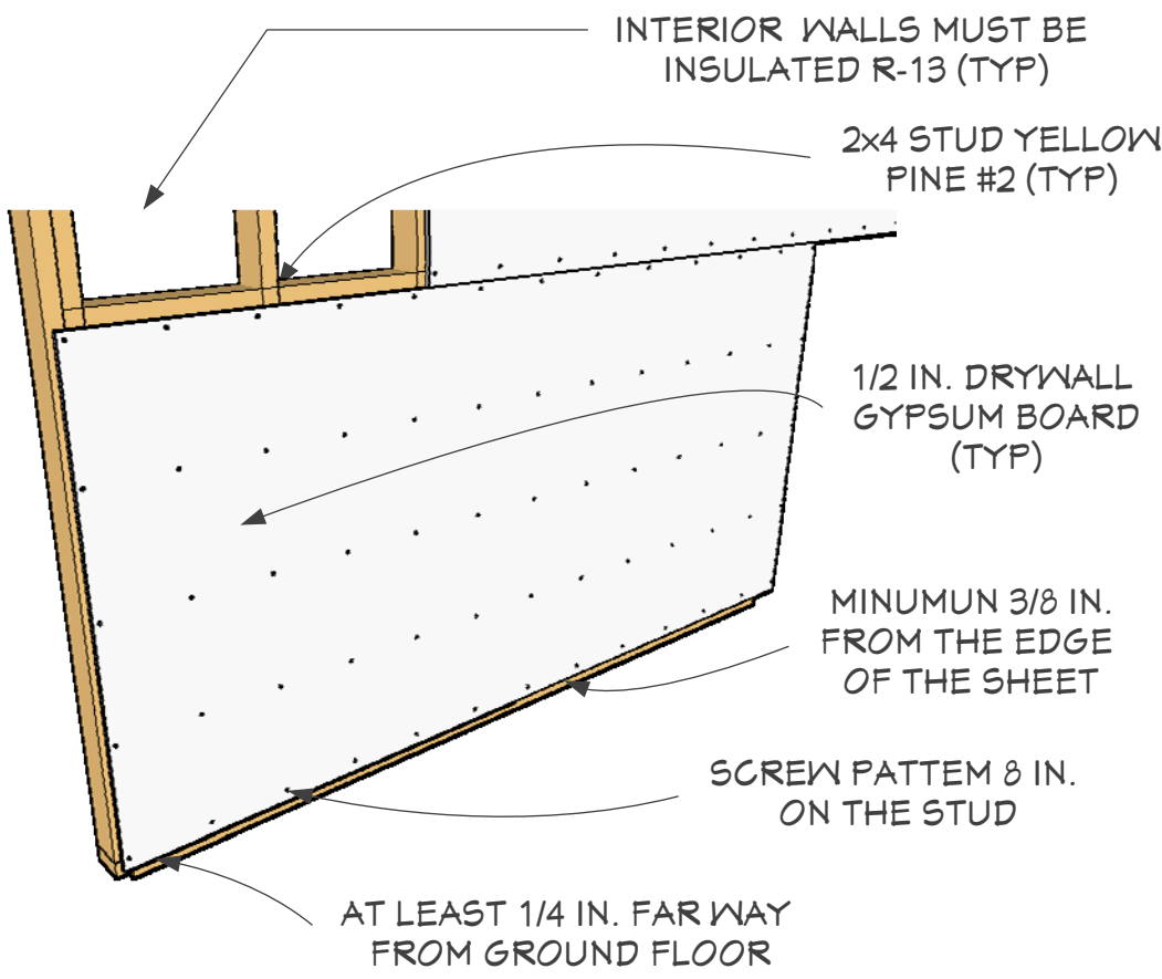
INTERIOR WALL DETAIL (TYP.)
