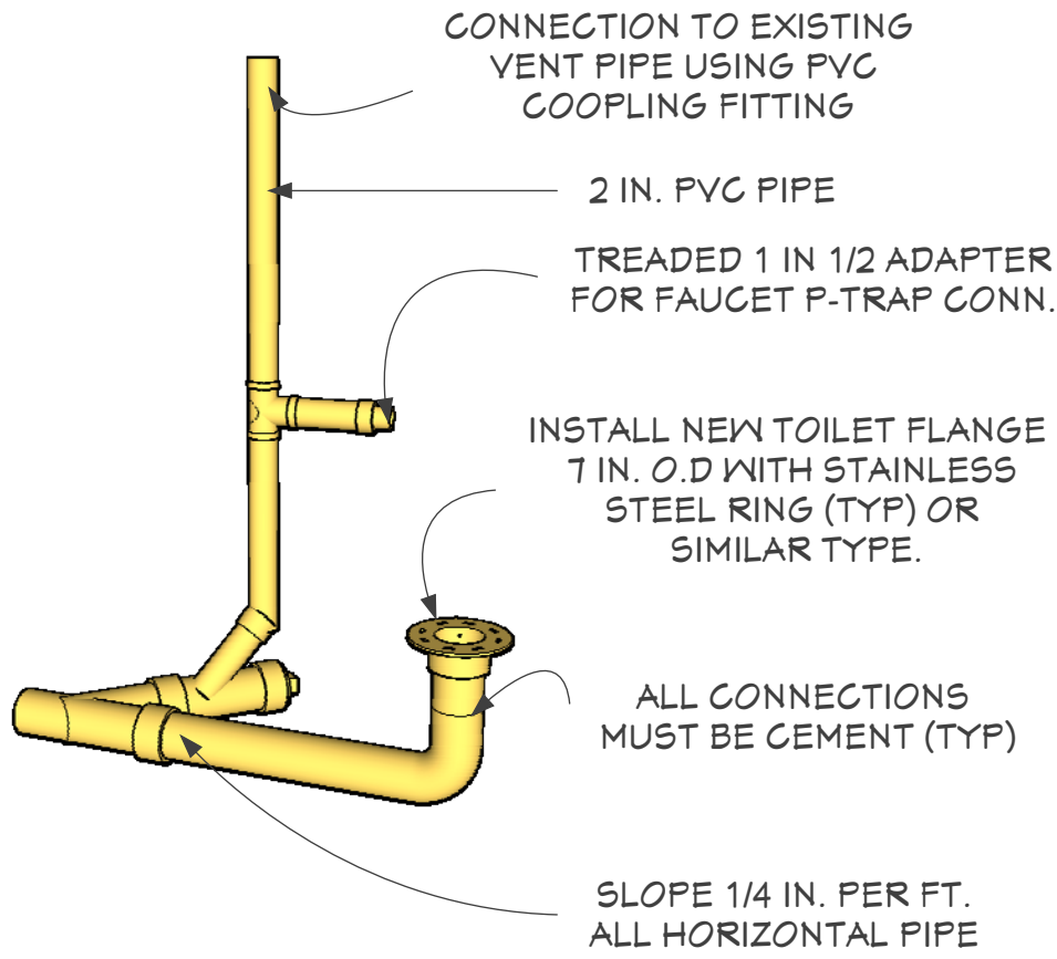
PLUMBING DRAIN PIPE DETAIL
